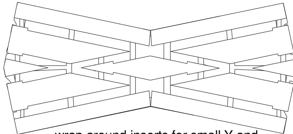
wrap around inserts for small Y and short crossing, OO Peco geometry
